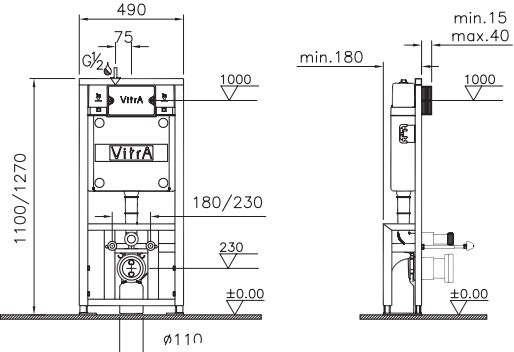
Regular Frame for Wall-hung WC Pans, back to back 742-5805-01 - 3/6 litre
